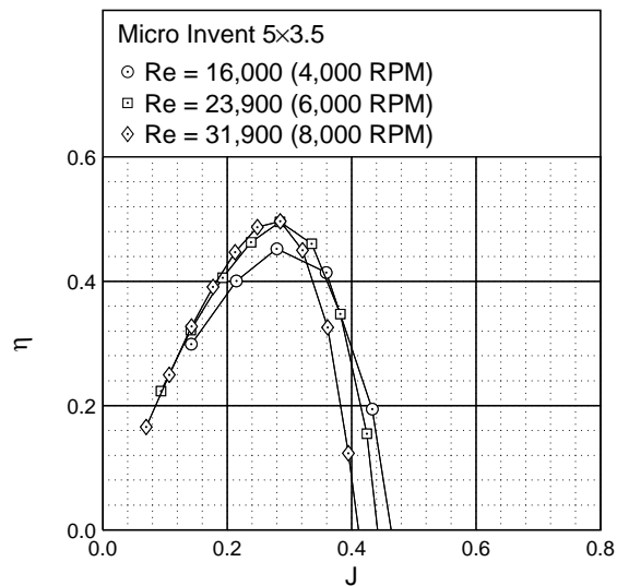
Figure 57: Micro Invent 5x3.5 efficiency curves.
