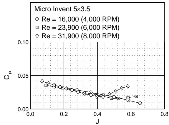
Figure 56: Micro Invent 5x3.5 power coefficient.
