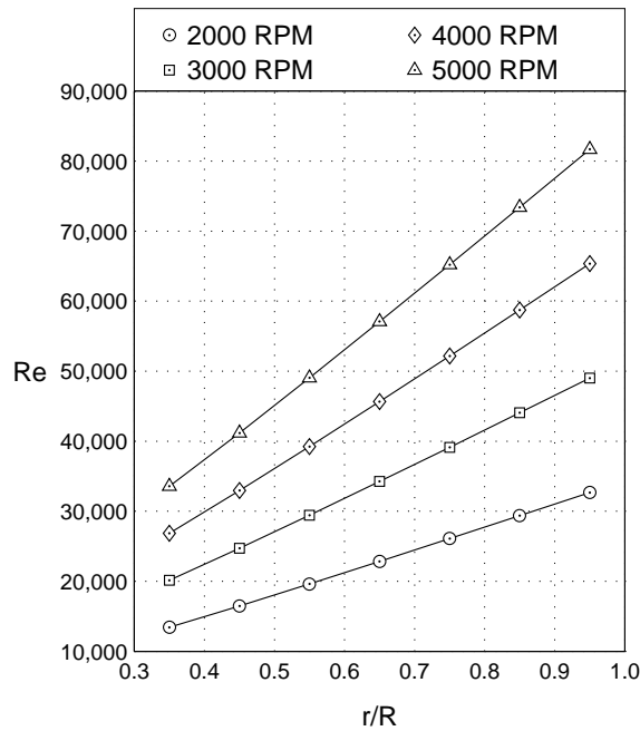
Figure 32: Reynolds number variation along the propeller blade for the DA4002 9×6.75 at an advance ratio of 0.60.
