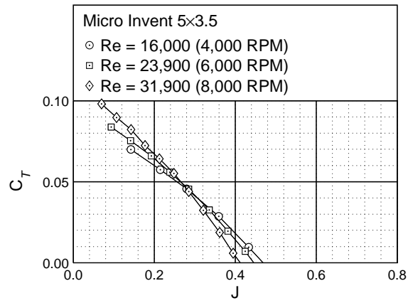
Figure 55: Micro Invent 5x3.5 thrust coefficient.
