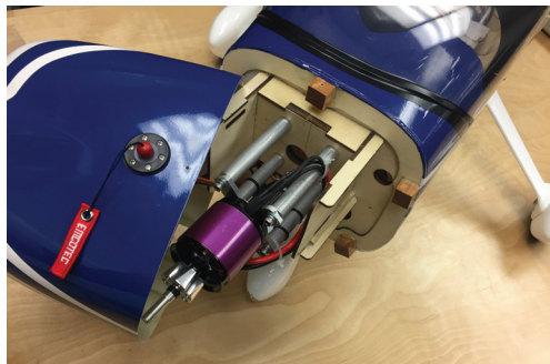
Figure 5. Hacker A50-14 L V3 motor mounted.
